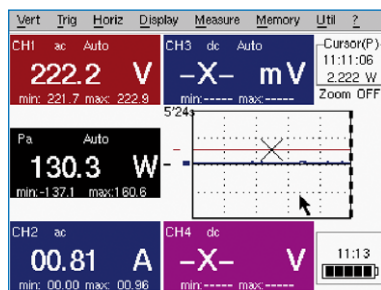
Display of active power and PF
