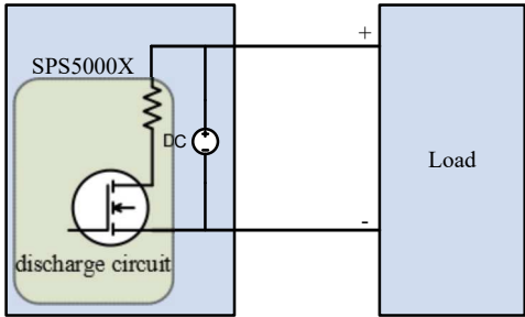
Discharge circuit
